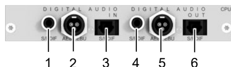
Fig. 22 Interface side L-/R474-BDD
