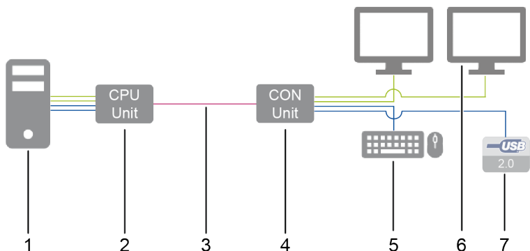
Fig. 7 Installation example (dual head with add-on module USB 2.0)
