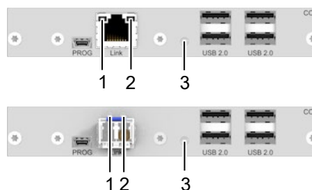
Fig. 52 Interface side USB 2.0 stand-alone modules - Failure indication
