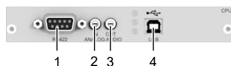
Fig. 18 Interface side L-/R474-BSE
