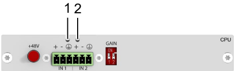
Fig. 38 Interface side add-on module balanced audio - Status LEDs L-/R474-BB2X
